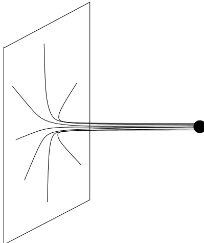
Figure 2: Charged particle placed into the bulk is connected to the brane by a string of gauge flux. The flux opens onto the brane as the field of a point charge.
